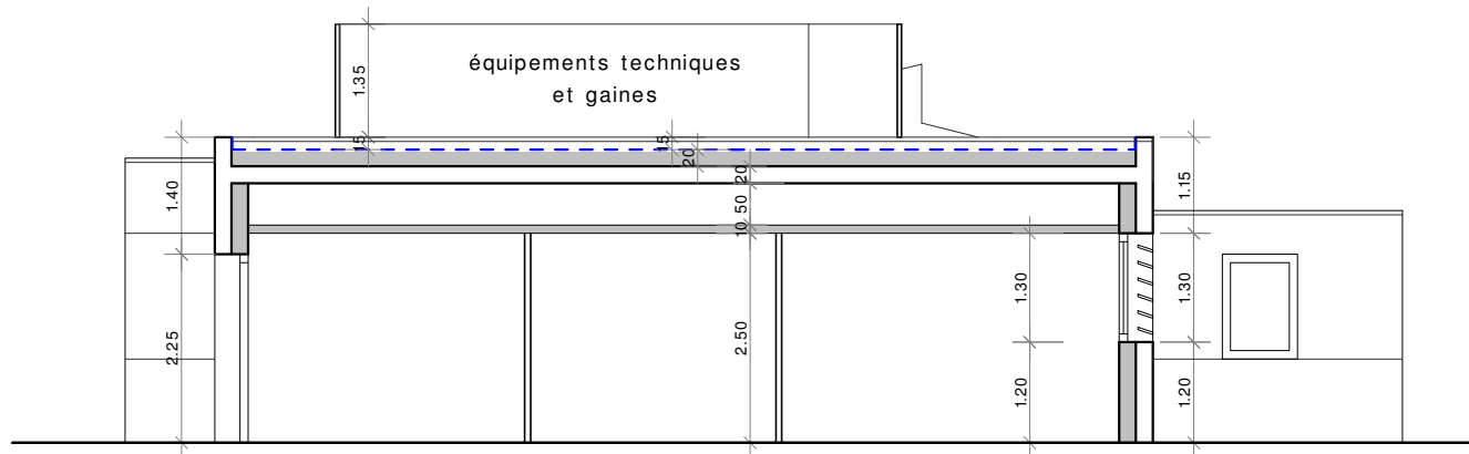
COUPE FACADE 5
